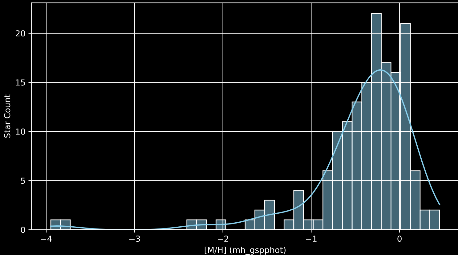
APOGEE DR17 Field: [K2_C11_007+09_btx [M/H] (mh_gspphot) (n= 159)
