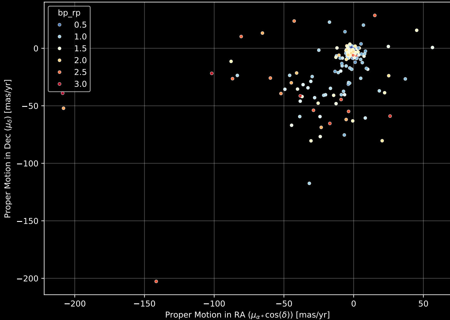
APOGEE DR17 Field: [K2_C11_007+09_btx] Proper Motion Diagram (n= 160)
