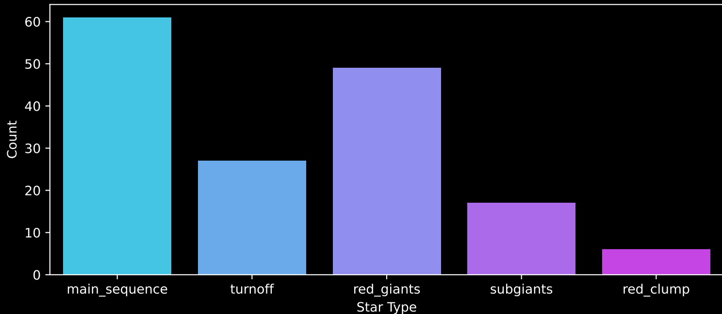
APOGEE DR17 Field: [K2_C11_007+09_btx] Count plot of Star Type
