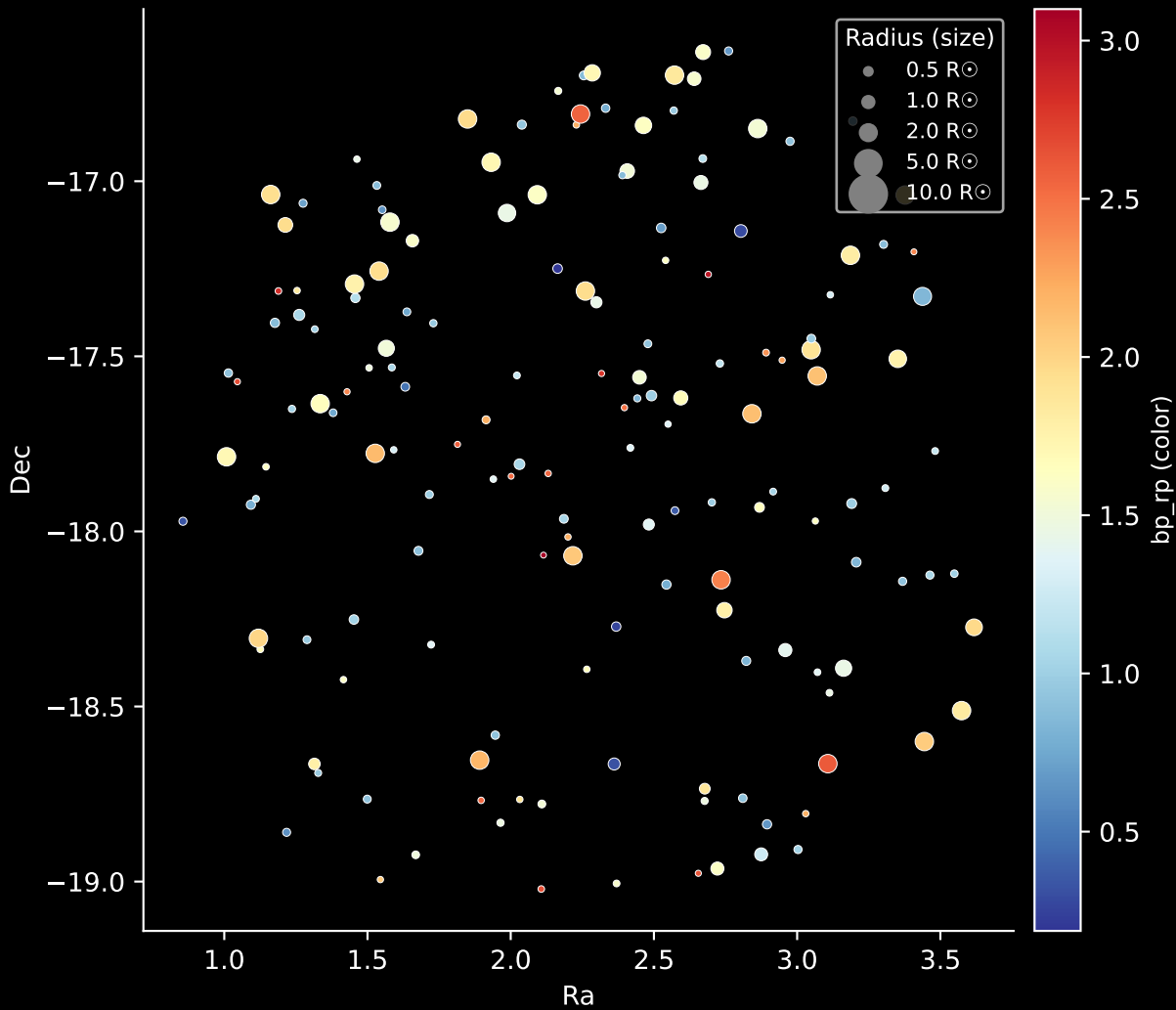
APOGEE DR17 Field: [K2_C11_007+09_btx] Stars: 160
