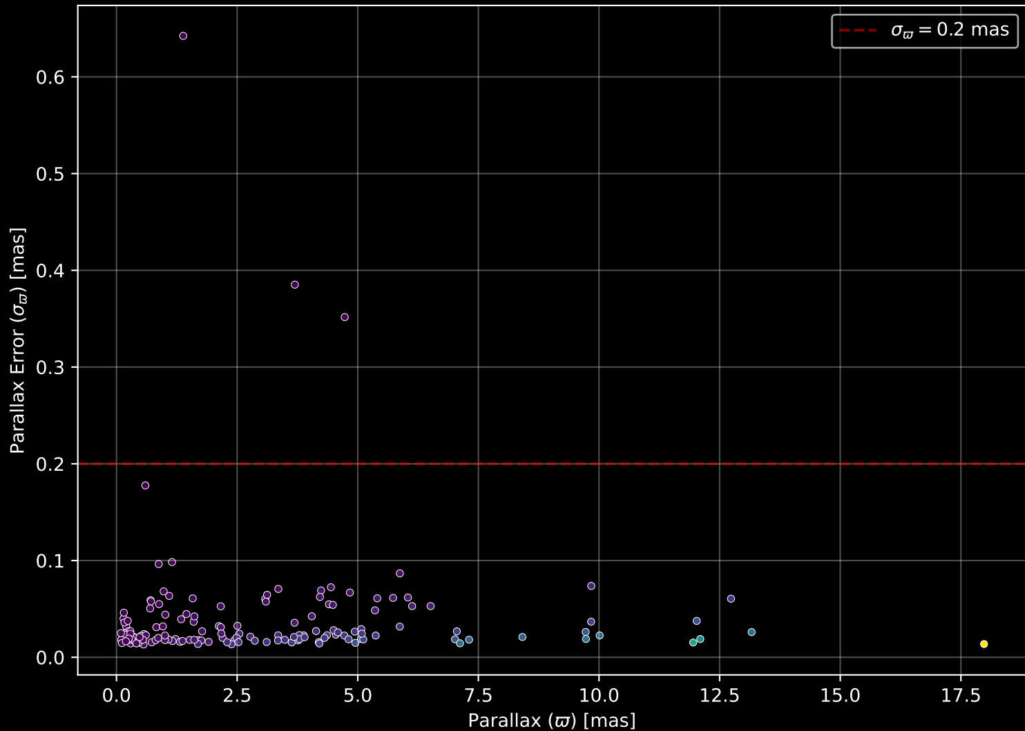
APOGEE DR17 Field: [K2_C11_007+09_btx] Parallax Quality (n= 160)
