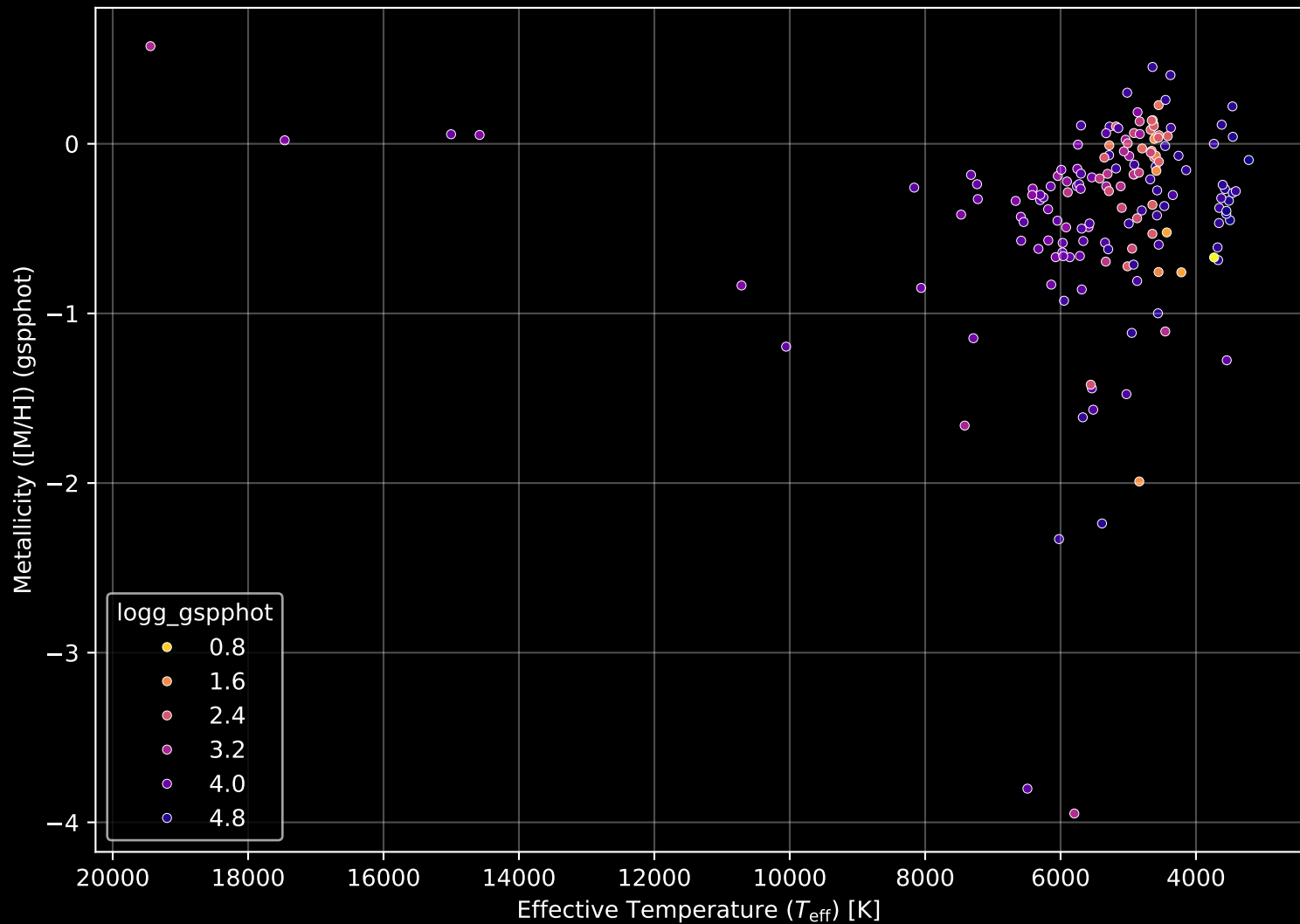
APOGEE DR17 Field: [K2_C11_007+09_btx] Stellar Population Parameters (n= 160)
