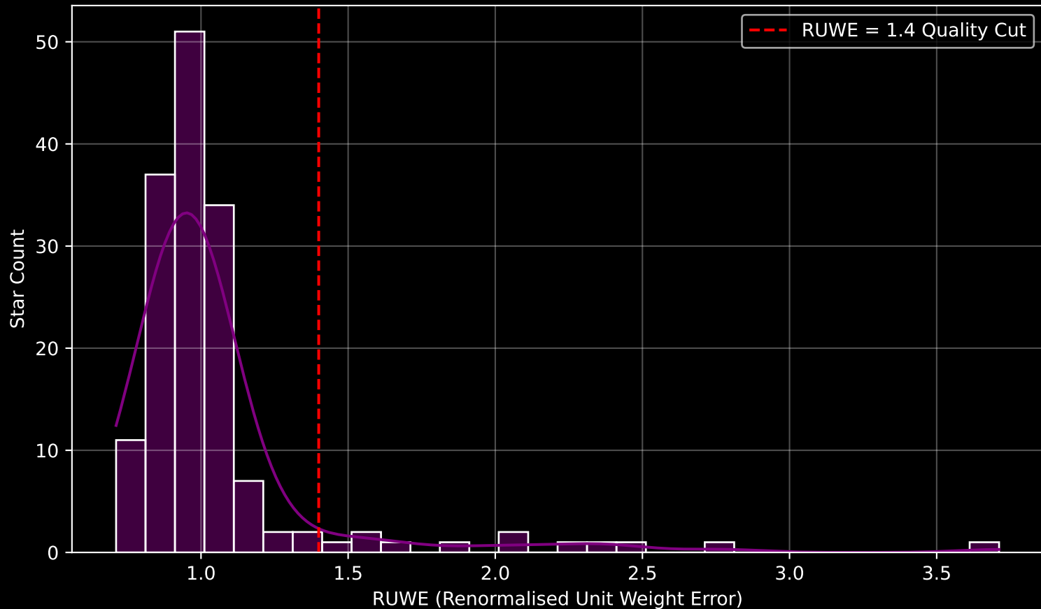
GAPOGEE DR17 Field [K2_C11_007+09_btx] RUWE Distribution (n= 156)
